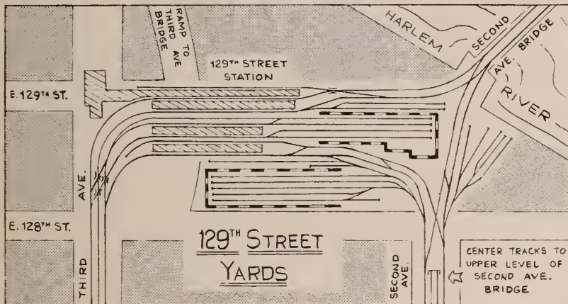
The 129th Street terminal and yard complex was built between 1886 and 1898 to serve both the Second and Third Avenue els as well as the Suburban line to The Bronx. The station was used to turn back local trains on both lines and thus served as a transfer point. UPPER LEFT: A view of the curve at Third Avenue and 129th Street in June 1940. A northbound train of Composites bound for The Bronx zips by the station and several trains of gate cars. George E. Votava. UPPER RIGHT: Looking west at the 129th Street terminal from Second Avenue. The platform at left was part of the yard and not open to passengers. George E.
